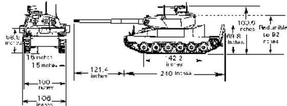
Figure 1-8. M1A2 characteristics.
