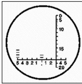
Figure 6-9. Mil scale in binocular reticle.
