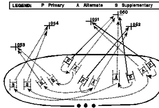
Figure 4-1. Fighting positions.
