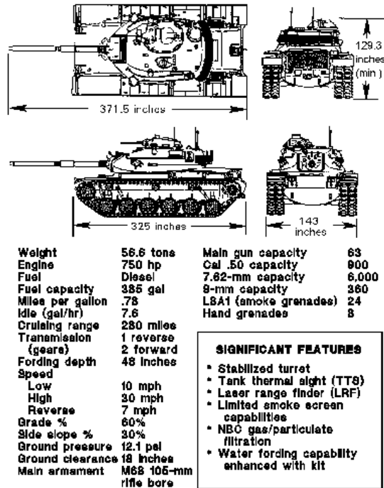
Figure 1-5. M60A3 characteristics.
